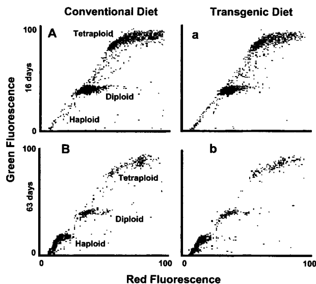
Fig. 1. Green vs. red fluorescence cytograms derived from 2000 AO-stained testicular cells from 16-day old mice fed (A) a conventional soybean diet and (a) a transgenic soybean diet. Diploid and tetraploid populations are apparent. Cytograms from (B) conventional and (b) transgenic soybean-fed 4th generation mice at 63 days after birth. Haploid cells comprise approximately 80% of total cells. There were no differences between treatments on the respective days.
